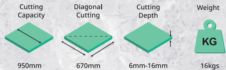
Sigillo 950mm Tile Cutter
